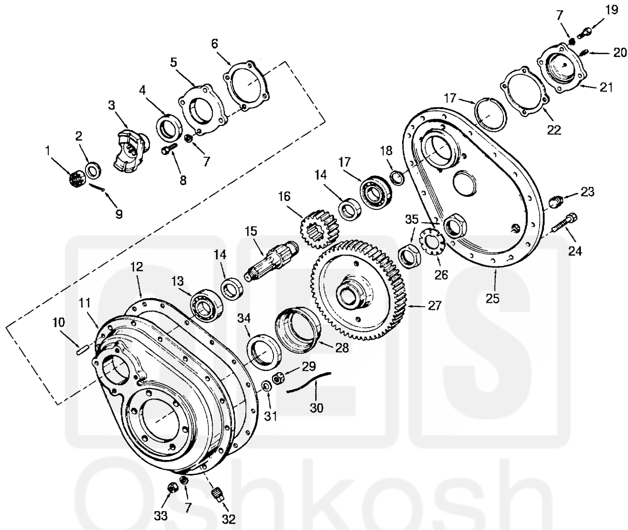
FIGURE 56. GEAR REDUCTION.
